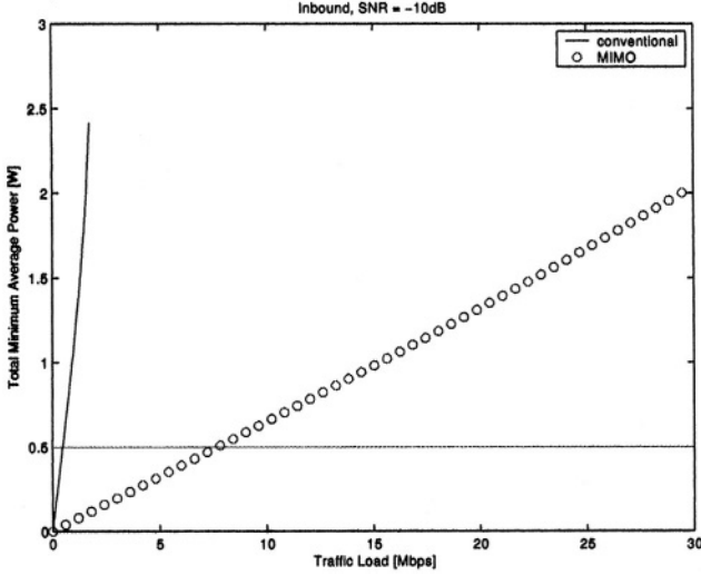
Figure 7: Inbound performance of a HCS. The total minimum average power H(C) is plotted as a function of the amount of traffic C that each node generates.
