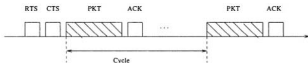
Figure 10: The MACA/PR protocol: RTS-CTS-PKT-ACK...PKT-ACK sequence. A CYCLE is the maximum interval allowed between two real-time packets.
