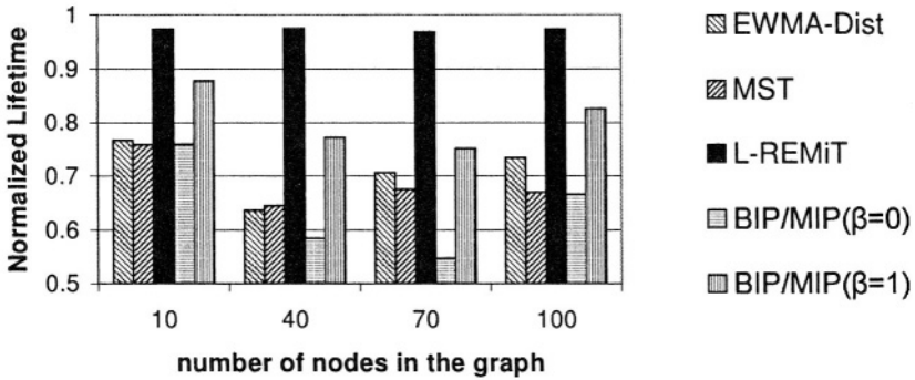
Figure 10: Average Normalized Lifetime for long range radios when 100% nodes are in multicast group for source-based multicast tree ( \alpha = 2, r_{max} = 10, K = 1, E^T = 0, E^R = 0 ).
