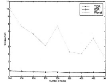
(e) IOR, TOR and WOR for random graph with \kappa = 2
