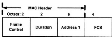
Figure 5: ACK format
