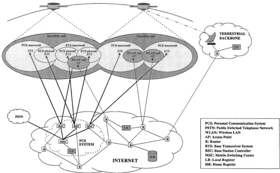
Figure 4: NGWS Architecture
