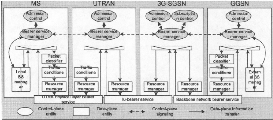
Figure 3: QoS Components in UMTS QoS Architecture
