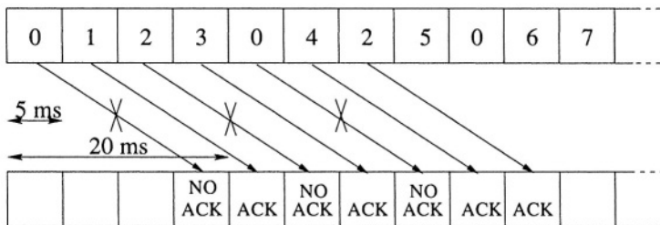
Figure 6: NARQP = 4 Timing
