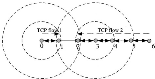
Figure 4: Node interference in a chain topology
