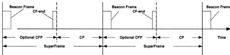
Figure 2: Superframes
