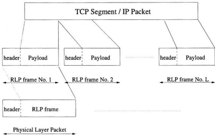
Figure 2: Fragmentation of TCP segments into RLP frames
