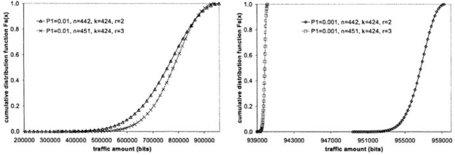
Figure 5: The Stochastic Service Curve for a Wireless Link
