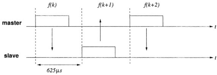
Figure 1: A snapshot of a Bluetooth frame.
