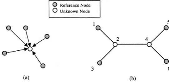
Figure 7: Examples of Multilateration [1].
