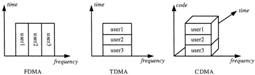
Figure 1: FDMA/TDMA/CDMA
