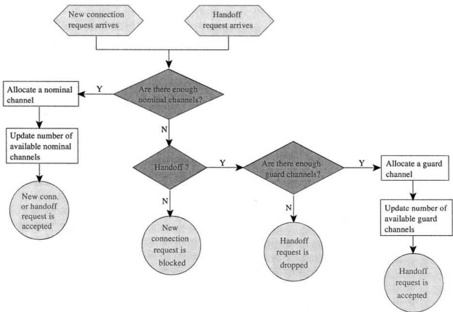
Figure 1: Generic CAC with Reservations
