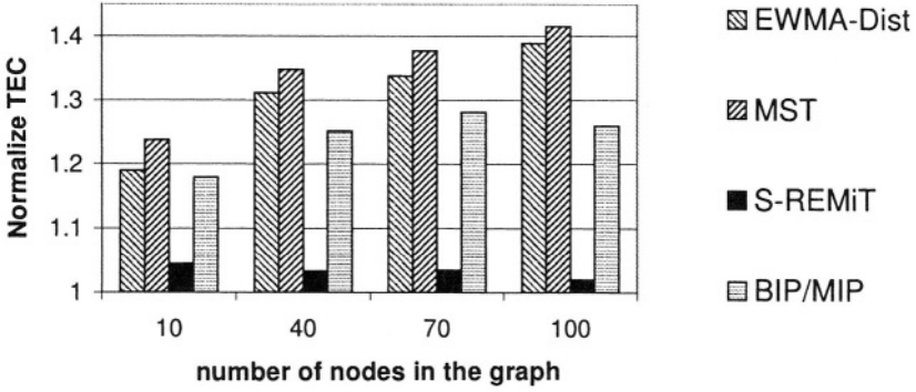
Figure 8: Average Normalized TEC for long range radios when 50% nodes are in multicast group for source-based multicast tree ( \alpha = 2, r_{max} = 10, K = 1, E^T = 0, E^R = 0.1 * K(r_{max})^\alpha ).
