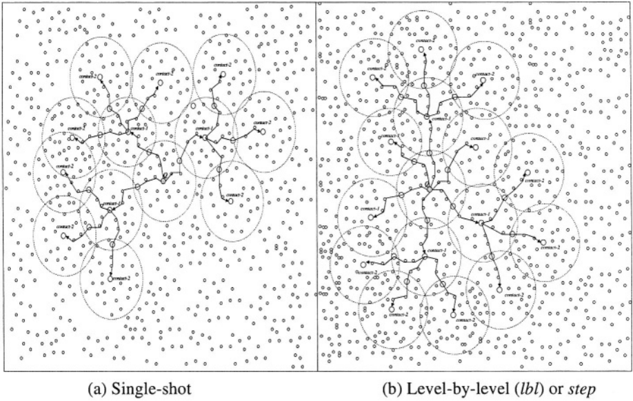
Figure 11: Examples of search policies with D = 2 , R = r = NoC = 3 : (a) The single-shot policy forwards the request in one attempt reaching level-1 and level-2 contacts (called contact-1 and contact-2), (b) The level-by-level ( lbl ) policy forwards the request in multiple attempts with increasing the visited levels. In the first attempt only ‘3’ level-1 contacts are visited. In the second attempt 3 different level-1 contacts are visited and the request is forwarded to ‘9’ level-2 contacts. It is clear that different policies reach different parts of the network. Single-shot may not be able to achieve good coverage near Q with low NoC .
