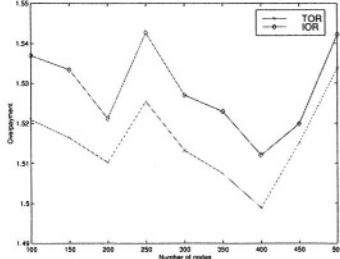
(a) IOR and TOR's difference for UDG with \kappa = 2
