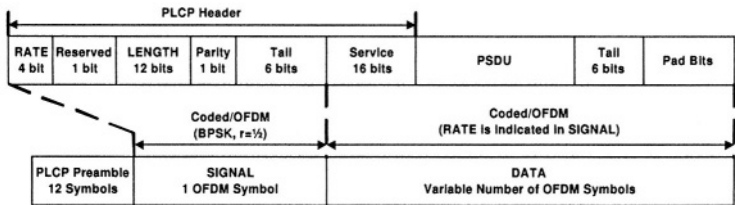
Figure 1: The PHY frame format for the IEEE 802.11a
